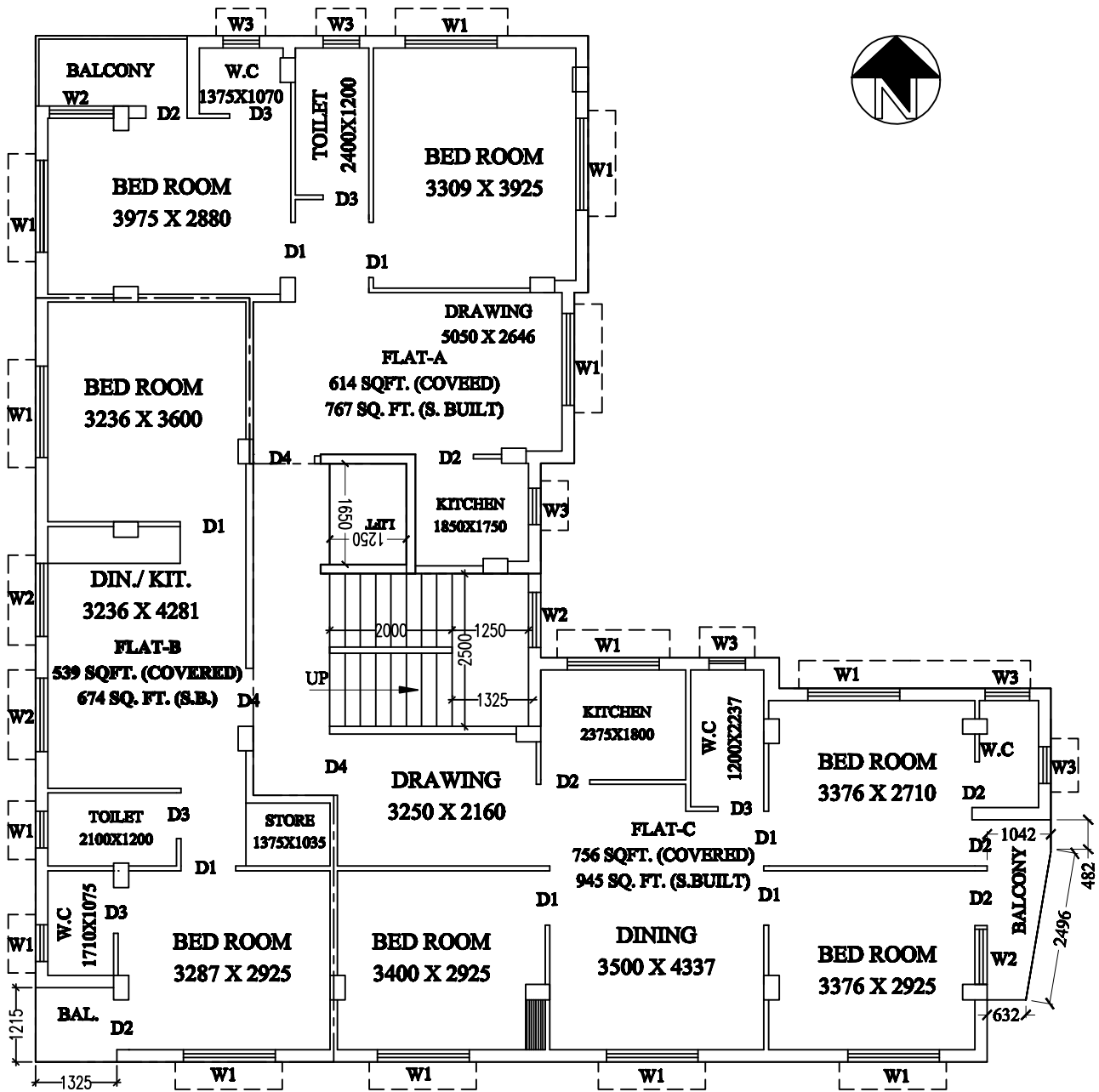
(TYP.) FLOOR PLAN
